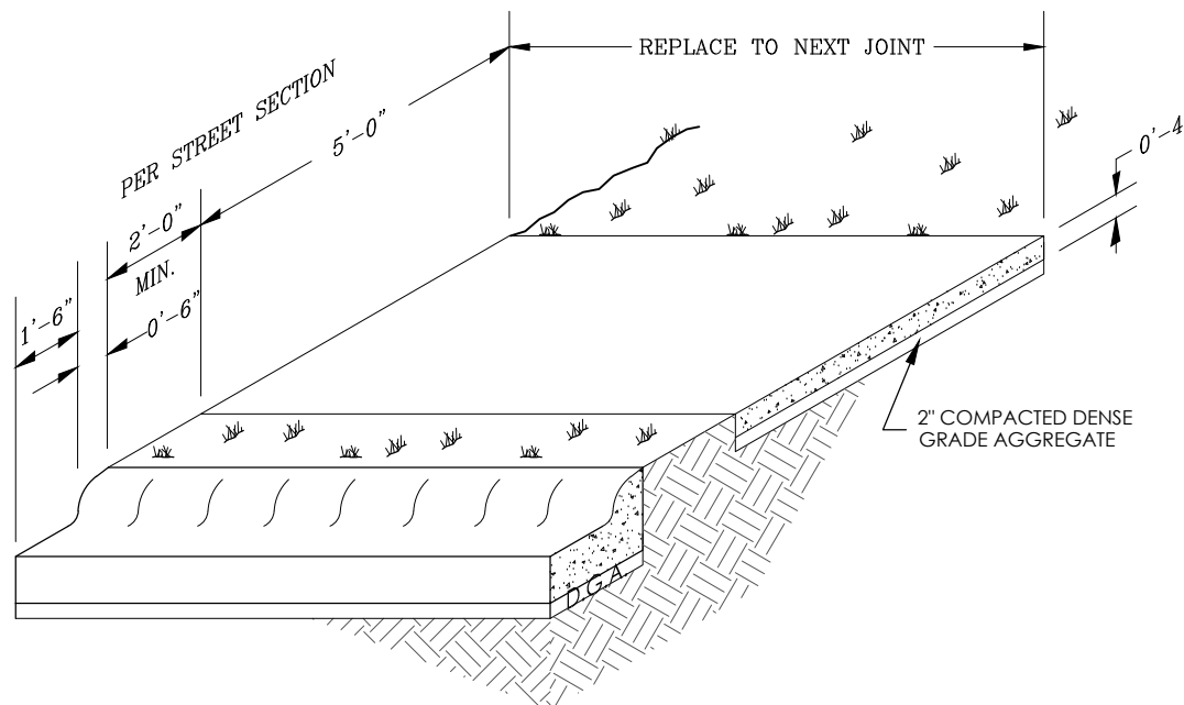
SIDEWALK DETAIL (TYPICAL SECTION) (N.T.S)
