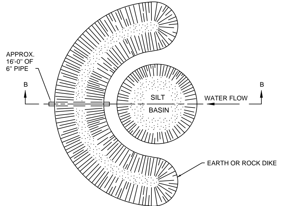
SILT TRAP TYPE B
