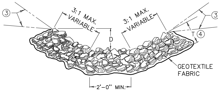
TYPICAL SECTION
