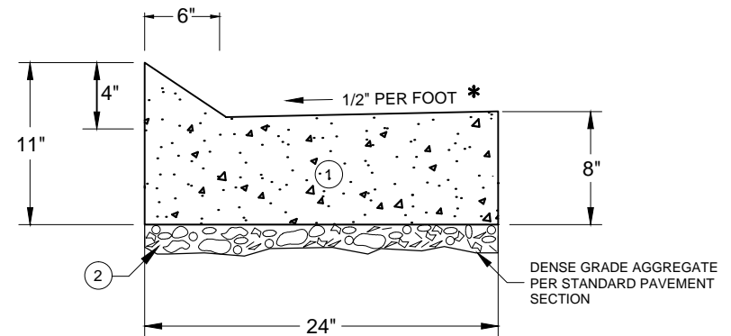
TYPICAL SECTION
