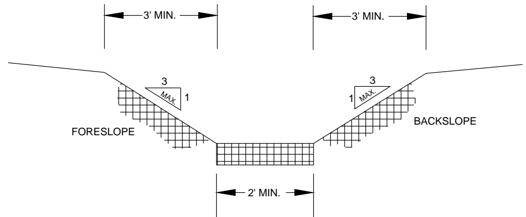
SODDED FLAT BOTTOM DITCH
