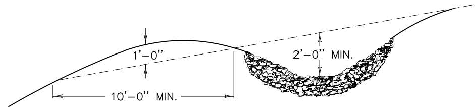
TYPICAL INTERCEPTOR DITCH
