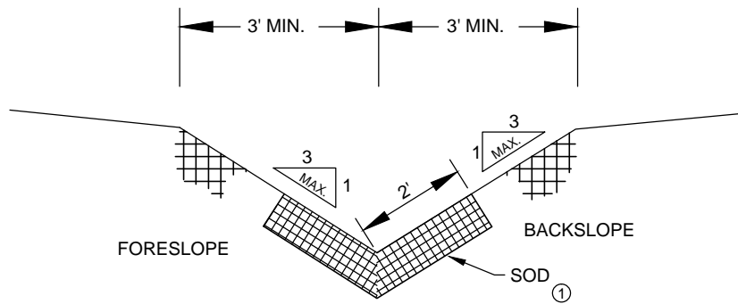
SODDED "V" DITCH
