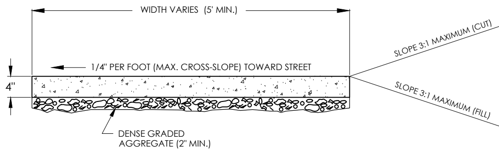
SIDEWALK DETAIL (TYPICAL SECTION) (N.T.S)
