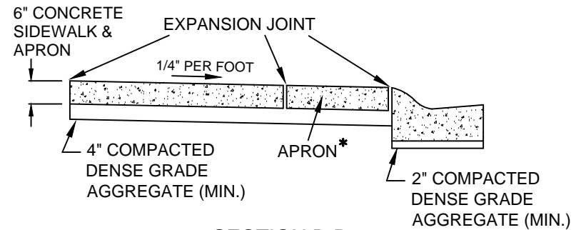
SECTION B-B
