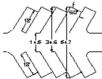
60° ANGLE PARKING* (ONE WAY TRAFFIC)
