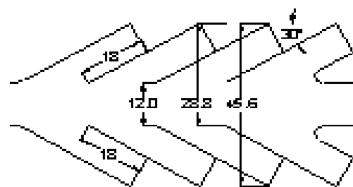
30° ANGLE PARKING* (ONE WAY TRAFFIC)
